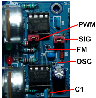
Fig 1b: Jumper & Solder Connections
